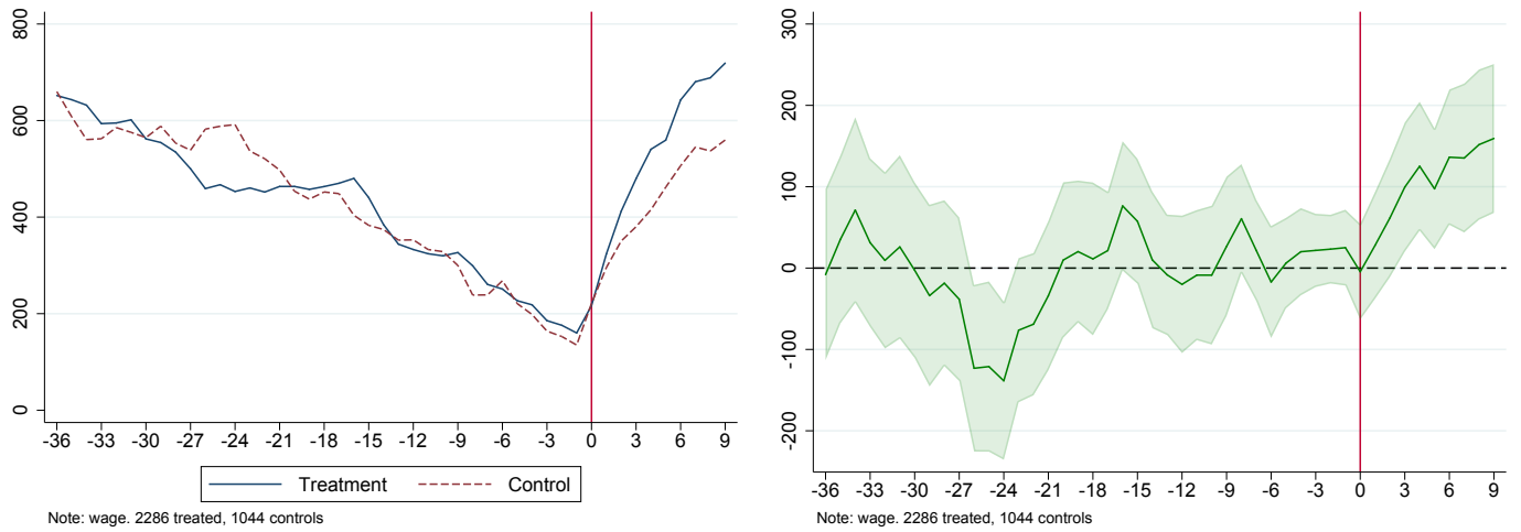
Figure 3: Monthly earnings
