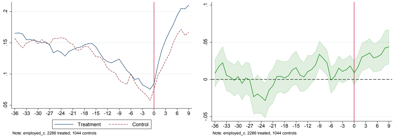
Figure 2: Employment
